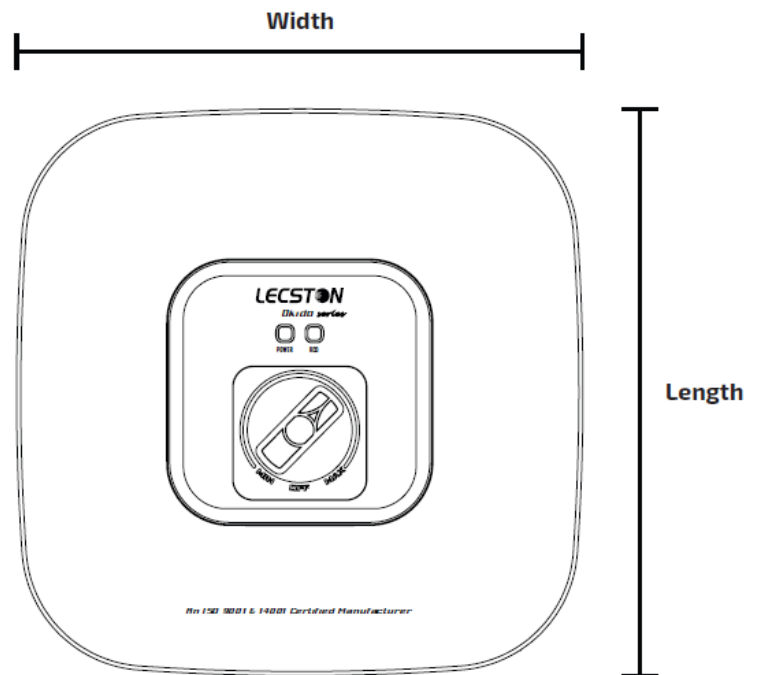
Okido OK707 Heater Dimension: 270mm (W) x 270mm (W) x 91mm (H)
